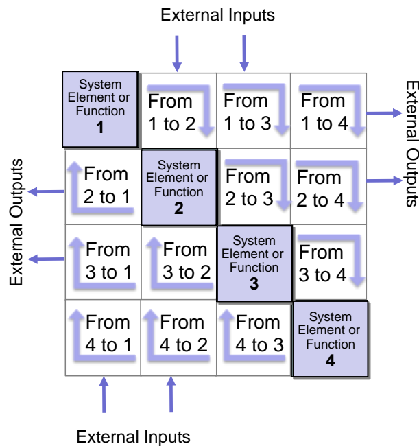
Figure 3: The key features and rules of an N^2 matrix
