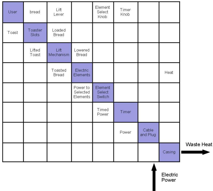
Figure 14: An N 2 Matrix for the Typical Domestic Toaster.
