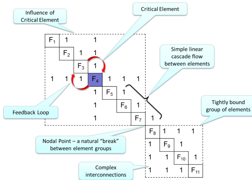
Figure 4: Possible N^2 Matrix Features
