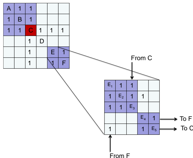
Figure 2: The top-down application of N^2 Analysis
